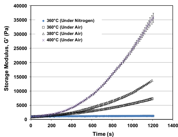
Fig. 7. Storage modulus versus time behavior of solution processed PEEK with 1% weight CNF under air and N 2 for different temperatures ( \omega = 1 rps).
