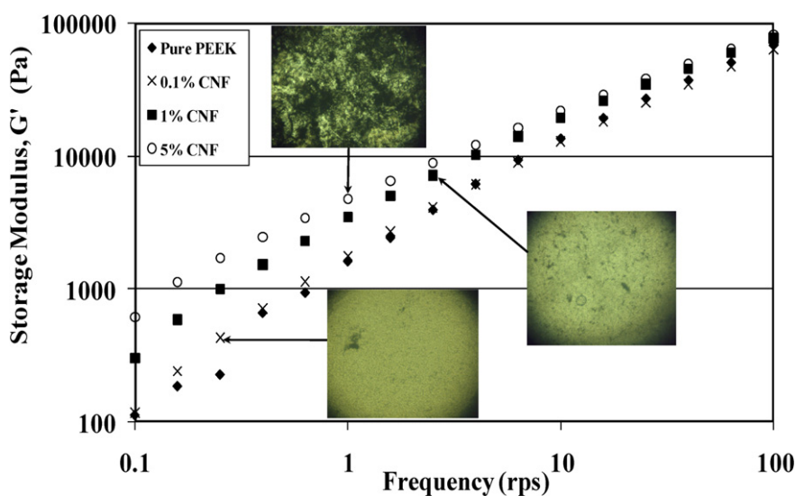
Fig. 9. Storage modulus versus frequency of solution processed PEEK and PEEK/CNF suspensions at 360 °C (insets show optical micrographs of solvent/CNF/PEEK mixtures).
