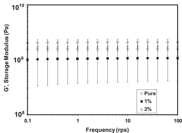
Fig. 2. Storage modulus of melt-compounded PEEK/CNF nanocomposites at ambient temperature.
