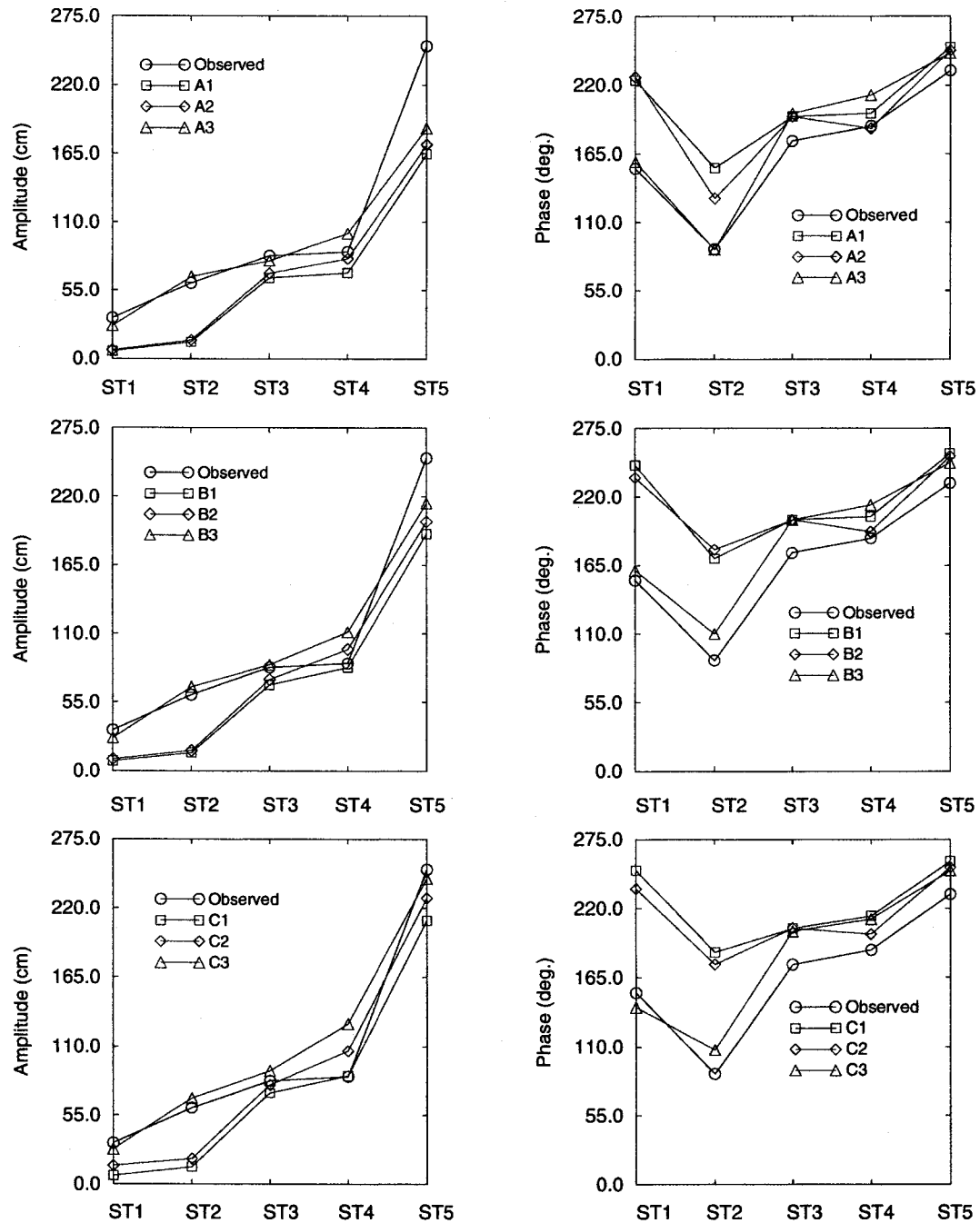
FIG. 2. The results of simulations with the Yellow Sea model for selected tidal stations (ST1–ST5). Amplitudes (left) and phases (right) for runs A1–A3 (Table 1) are presented on the upper panel; for runs B1–B3, the middle panel; and for C1–C3, the bottom panel. The curves marked with a circle are the observed amplitudes and phases (relative to UTC); the curves marked with a square are the results of runs A1, B1, and C1; the curves marked with a rhombus are the results of runs A2, B2, and C2; and the curves marked with a triangle are the results of runs A3, B3, and C3.
