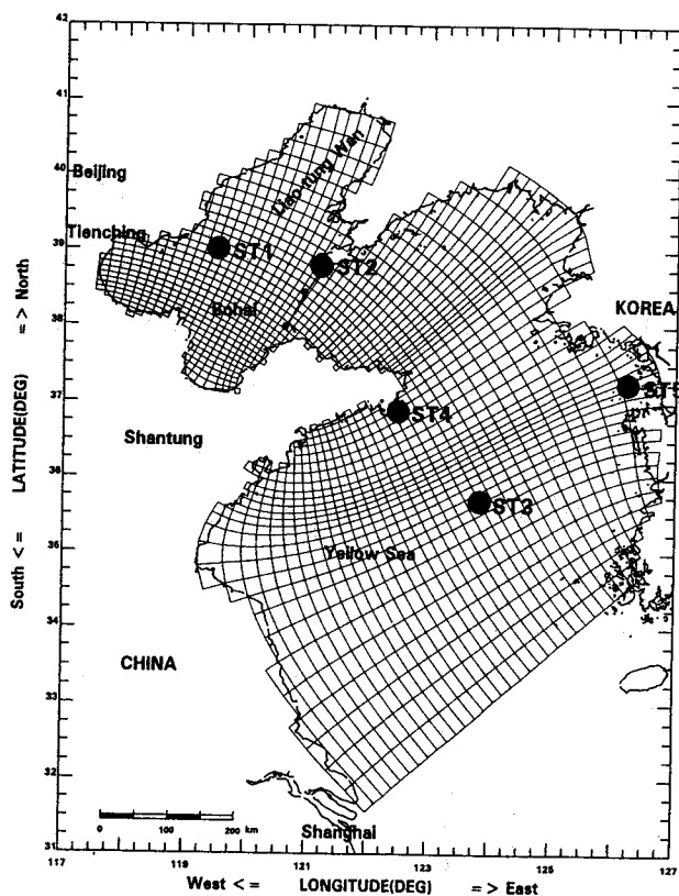
FIG. 1. Curvilinear orthogonal model grid of the Yellow Sea. ST1–ST5 are tidal stations.
